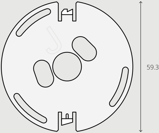
Backplate
